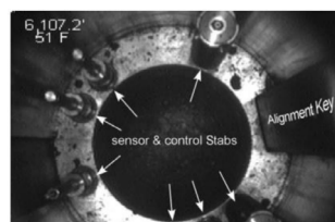
Tubing Hanger control stabs inspection
